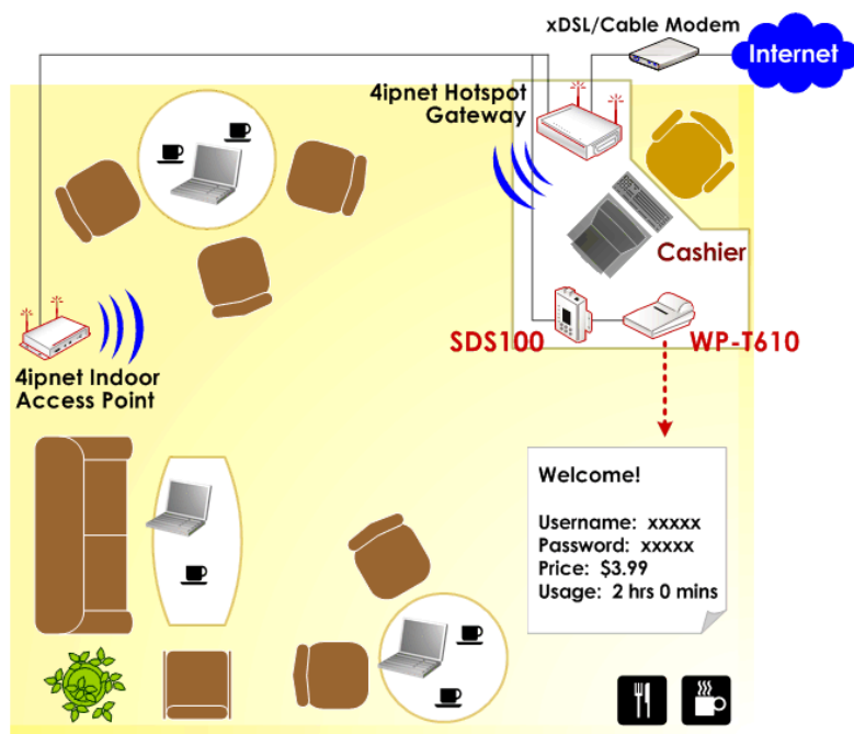
Small-size Hotspot Network
