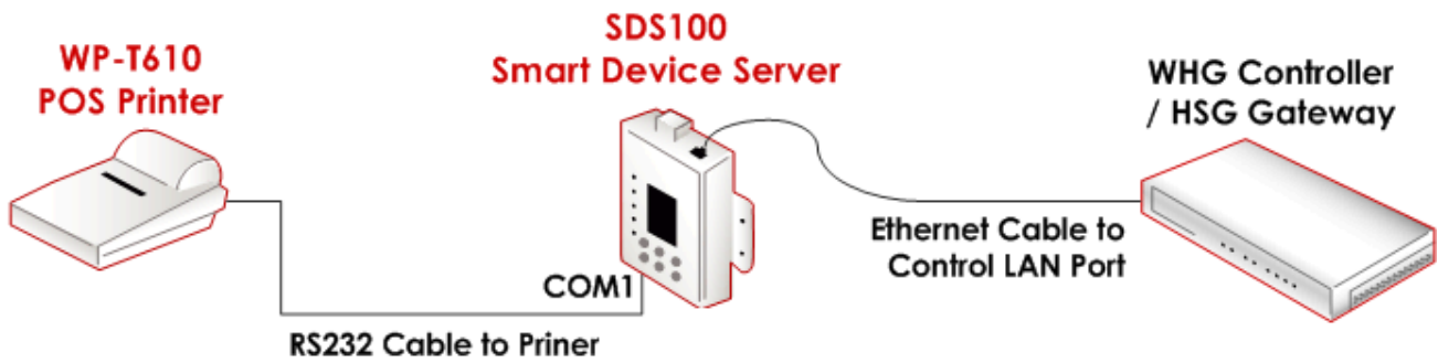
Diagram of SDS100 Connecting to WP-T610 and WHG Controller
